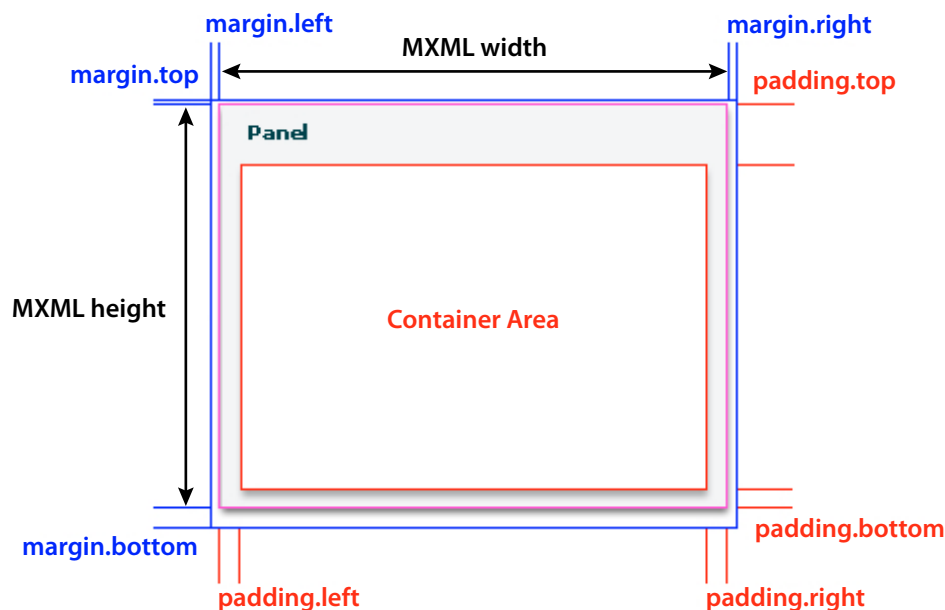
Margin and padding relationships in respect to a panel component
